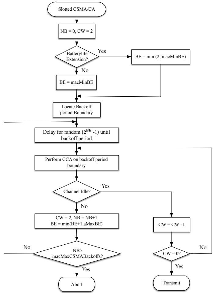
Fig. 4. IEEE 802.15.4 slotted CSMA/CA protocol flowchart [12].
